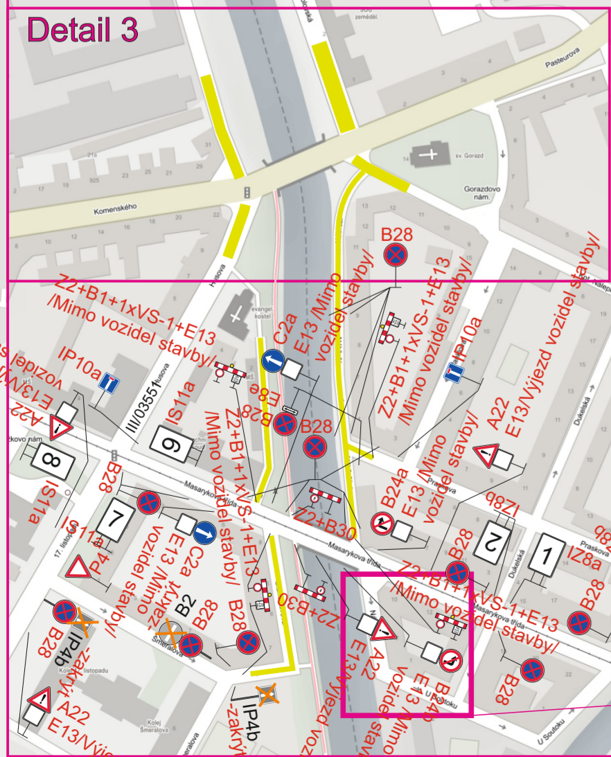
Detail 3
